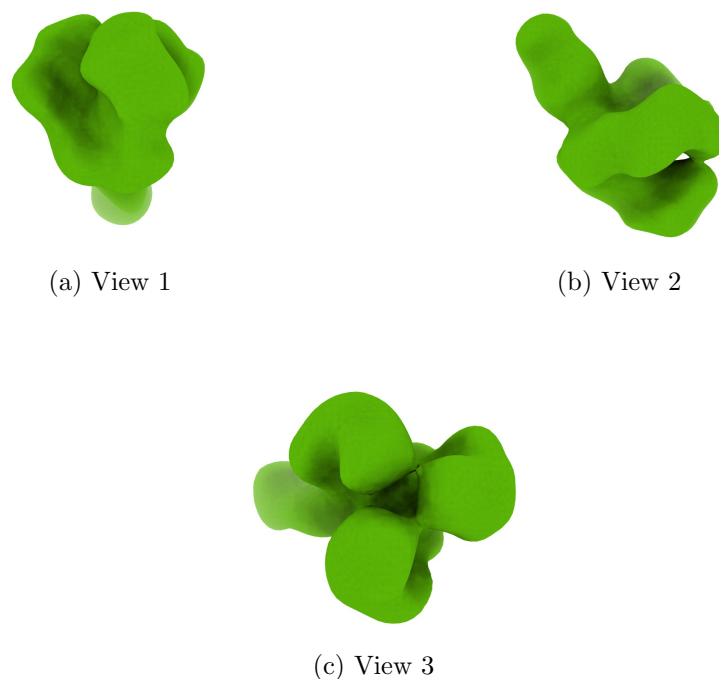
Figure 4: Isosurface at threshold=0.038800. Views generated by ChimeraX at a the following X, Y, Z angles: View 1 (0, -90, -90), View 2 (-90, 0, -90), View 3 (0, 0, 0).
