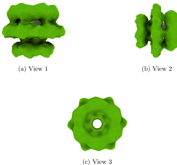
Figure 4: Isosurface at threshold=0.213000. Views generated by ChimeraX at a the following X, Y, Z angles: View 1 (0, -90, -90), View 2 (-90, 0, -90), View 3 (0, 0, 0).
