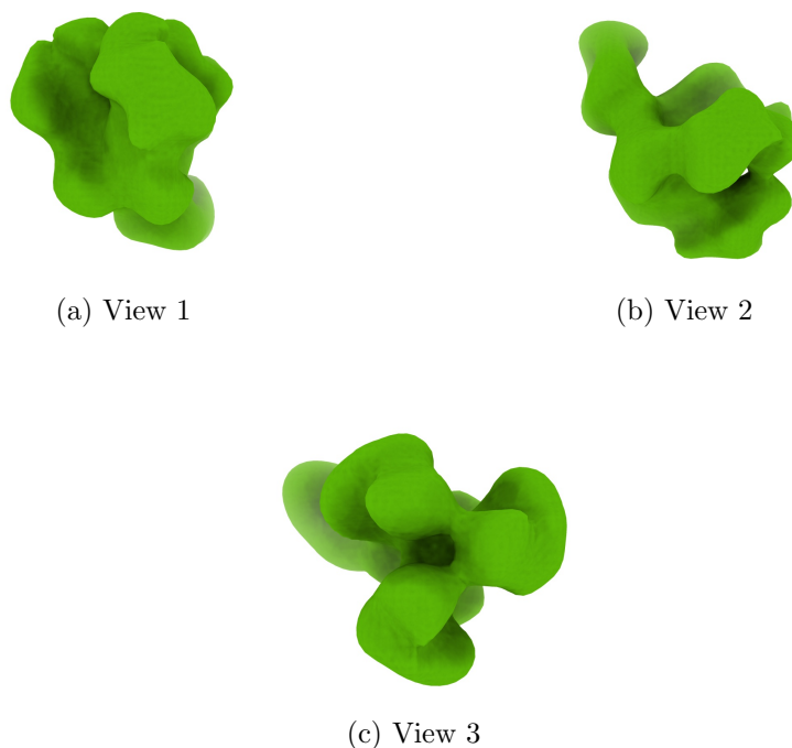
Figure 4: Isosurface at threshold=0.049200. Views generated by ChimeraX at a the following X, Y, Z angles: View 1 (0, -90, -90), View 2 (-90, 0, -90), View 3 (0, 0, 0).
