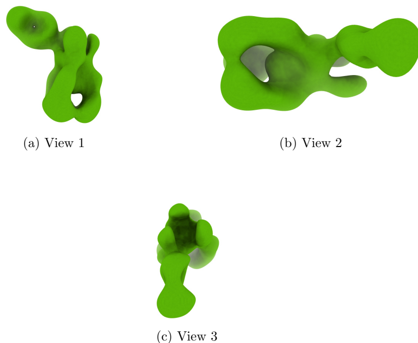
Figure 4: Isosurface at threshold=0.031000. Views generated by ChimeraX at a the following X, Y, Z angles: View 1 (0, -90, -90), View 2 (-90, 0, -90), View 3 (0, 0, 0).
