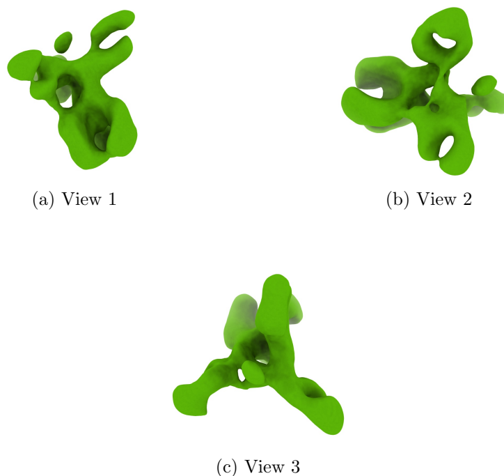
Figure 4: Isosurface at threshold=0.018700. Views generated by ChimeraX at a the following X, Y, Z angles: View 1 (0, -90, -90), View 2 (-90, 0, -90), View 3 (0, 0, 0).
