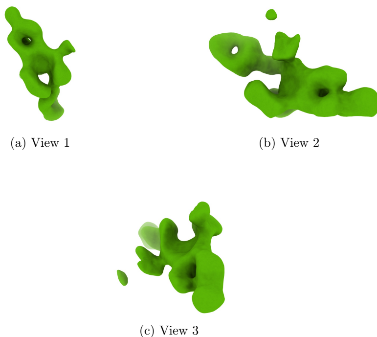
Figure 4: Isosurface at threshold=0.020700. Views generated by ChimeraX at a the following X, Y, Z angles: View 1 (0, -90, -90), View 2 (-90, 0, -90), View 3 (0, 0, 0).
