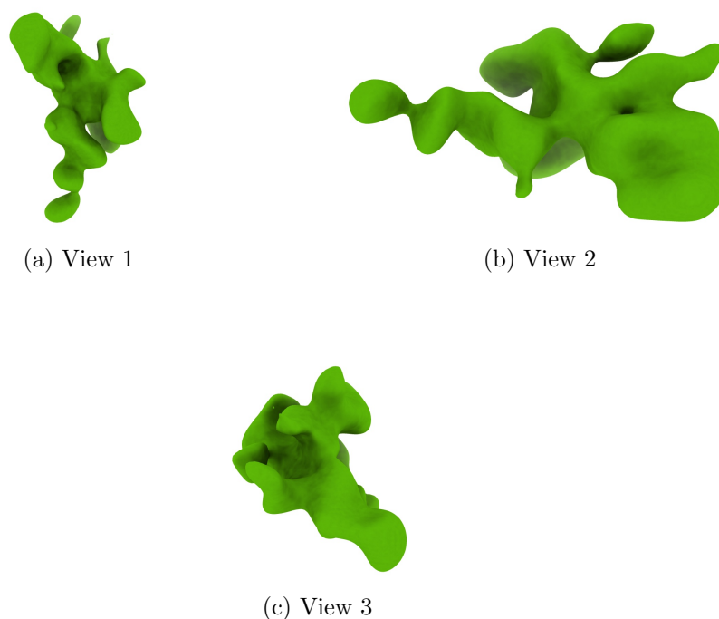
Figure 4: Isosurface at threshold=0.016000. Views generated by ChimeraX at a the following X, Y, Z angles: View 1 (0, -90, -90), View 2 (-90, 0, -90), View 3 (0, 0, 0).
