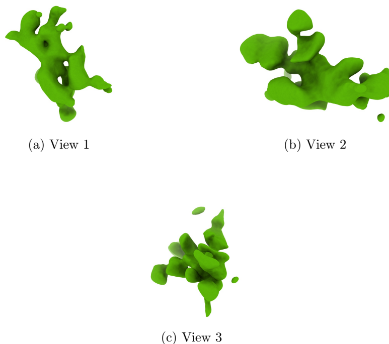
Figure 4: Isosurface at threshold=0.015100. Views generated by ChimeraX at a the following X, Y, Z angles: View 1 (0, -90, -90), View 2 (-90, 0, -90), View 3 (0, 0, 0).
