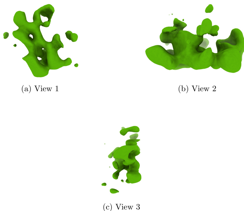
Figure 4: Isosurface at threshold=0.014800. Views generated by ChimeraX at a the following X, Y, Z angles: View 1 (0, -90, -90), View 2 (-90, 0, -90), View 3 (0, 0, 0).
