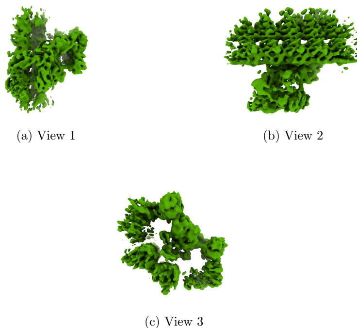
Figure 4: Isosurface at threshold=0.248000. Views generated by ChimeraX at a the following X, Y, Z angles: View 1 (0, -90, -90), View 2 (-90, 0, -90), View 3 (0, 0, 0).
