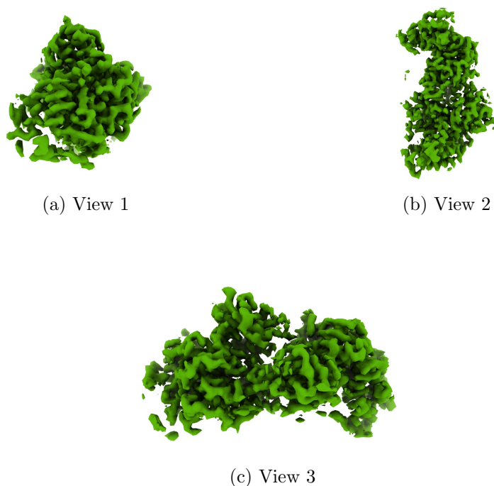
Figure 4: Isosurface at threshold=0.120000. Views generated by ChimeraX at a the following X, Y, Z angles: View 1 (0, -90, -90), View 2 (-90, 0, -90), View 3 (0, 0, 0).
