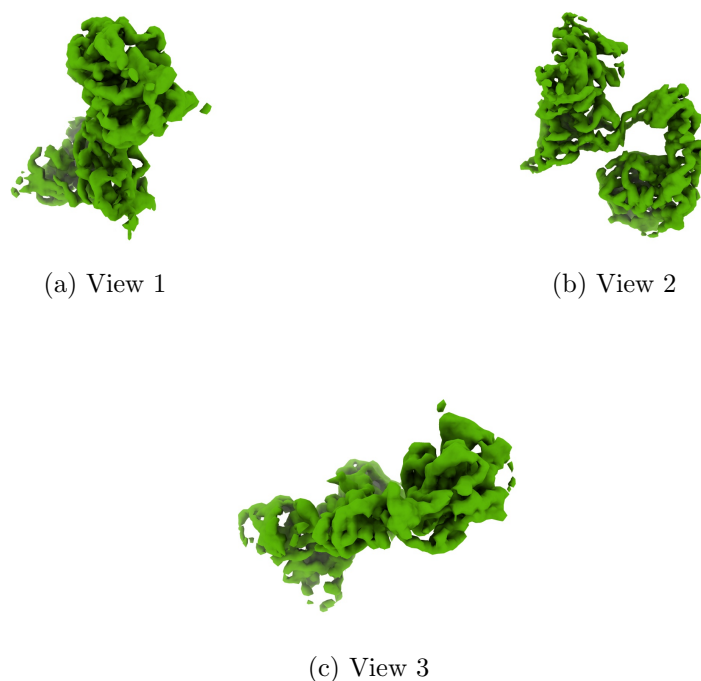
Figure 4: Isosurface at threshold=2.000000. Views generated by ChimeraX at a the following X, Y, Z angles: View 1 (0, -90, -90), View 2 (-90, 0, -90), View 3 (0, 0, 0).
