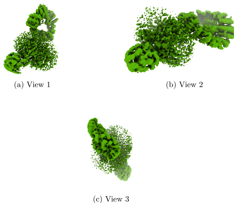
Figure 4: Isosurface at threshold=0.227000. Views generated by ChimeraX at a the following X, Y, Z angles: View 1 (0, -90, -90), View 2 (-90, 0, -90), View 3 (0, 0, 0).
