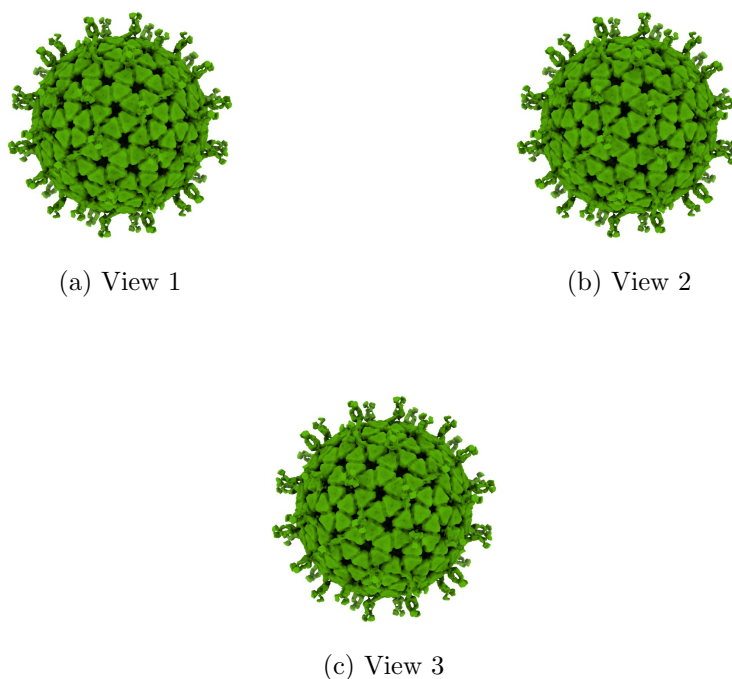
Figure 4: Isosurface at threshold=2.460000. Views generated by ChimeraX at a the following X, Y, Z angles: View 1 (0, -90, -90), View 2 (-90, 0, -90), View 3 (0, 0, 0).
