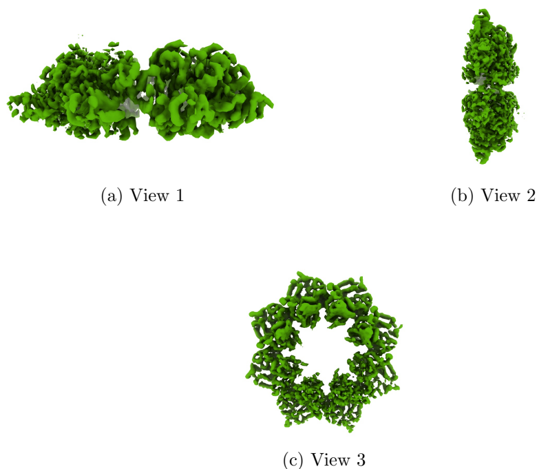
Figure 4: Isosurface at threshold=0.221000. Views generated by ChimeraX at a the following X, Y, Z angles: View 1 (0, -90, -90), View 2 (-90, 0, -90), View 3 (0, 0, 0).
