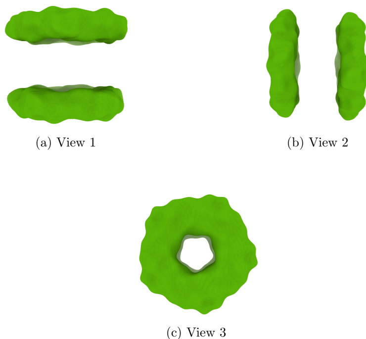
Figure 4: Isosurface at threshold=0.002800. Views generated by ChimeraX at a the following X, Y, Z angles: View 1 (0, -90, -90), View 2 (-90, 0, -90), View 3 (0, 0, 0).
