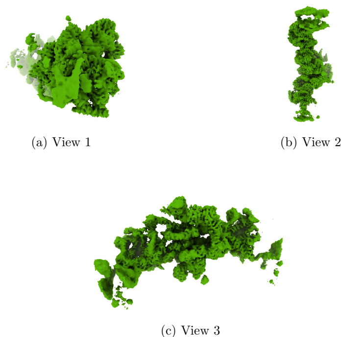
Figure 4: Isosurface at threshold=0.366000. Views generated by ChimeraX at a the following X, Y, Z angles: View 1 (0, -90, -90), View 2 (-90, 0, -90), View 3 (0, 0, 0).
