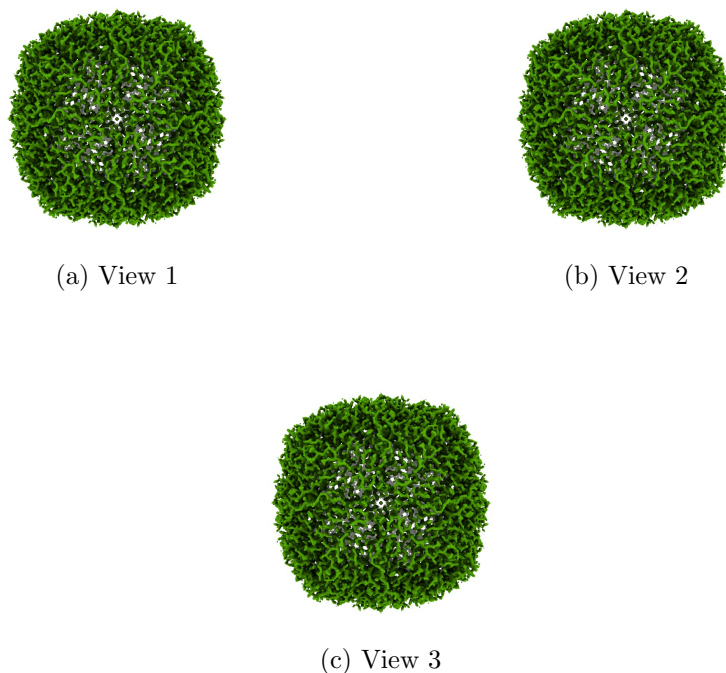
Figure 4: Isosurface at threshold=0.630000. Views generated by ChimeraX at a the following X, Y, Z angles: View 1 (0, -90, -90), View 2 (-90, 0, -90), View 3 (0, 0, 0).
