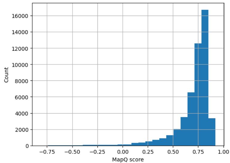
Figure 16: Histogram of the per-atom Q-score.
