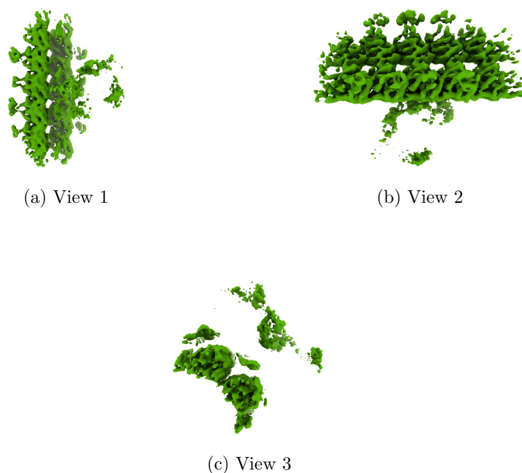
Figure 4: Isosurface at threshold=0.354000. Views generated by ChimeraX at a the following X, Y, Z angles: View 1 (0, -90, -90), View 2 (-90, 0, -90), View 3 (0, 0, 0).
