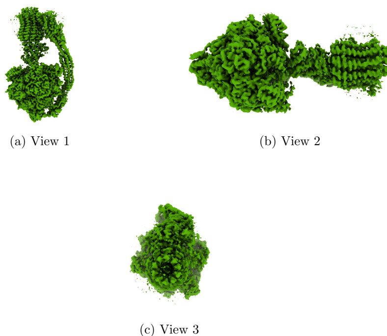
Figure 4: Isosurface at threshold=1.100000. Views generated by ChimeraX at a the following X, Y, Z angles: View 1 (0, -90, -90), View 2 (-90, 0, -90), View 3 (0, 0, 0).
