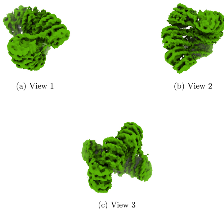
Figure 4: Isosurface at threshold=3.480000. Views generated by ChimeraX at a the following X, Y, Z angles: View 1 (0, -90, -90), View 2 (-90, 0, -90), View 3 (0, 0, 0).
