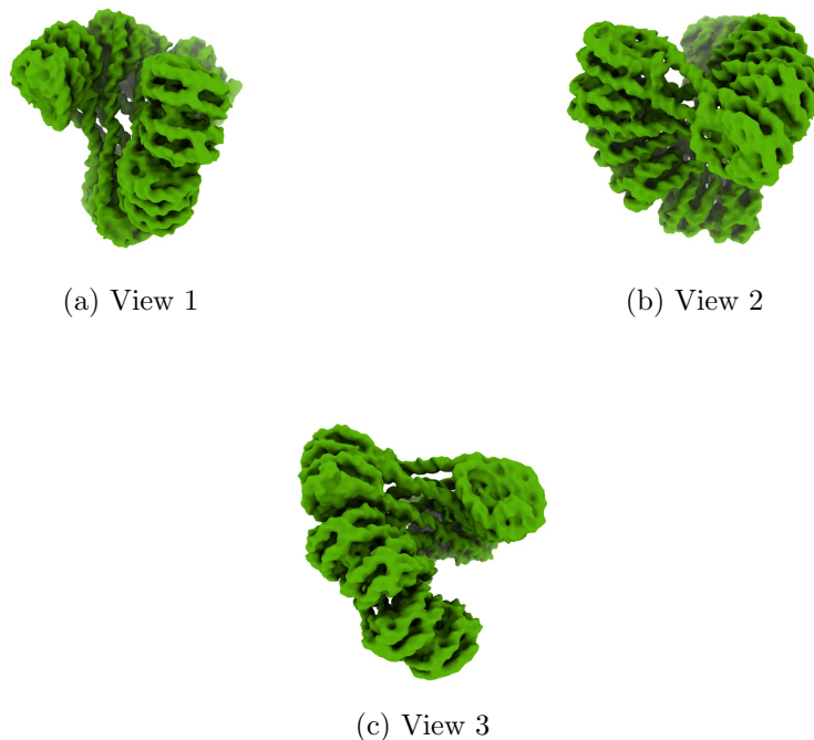
Figure 4: Isosurface at threshold=3.160000. Views generated by ChimeraX at a the following X, Y, Z angles: View 1 (0, -90, -90), View 2 (-90, 0, -90), View 3 (0, 0, 0).
