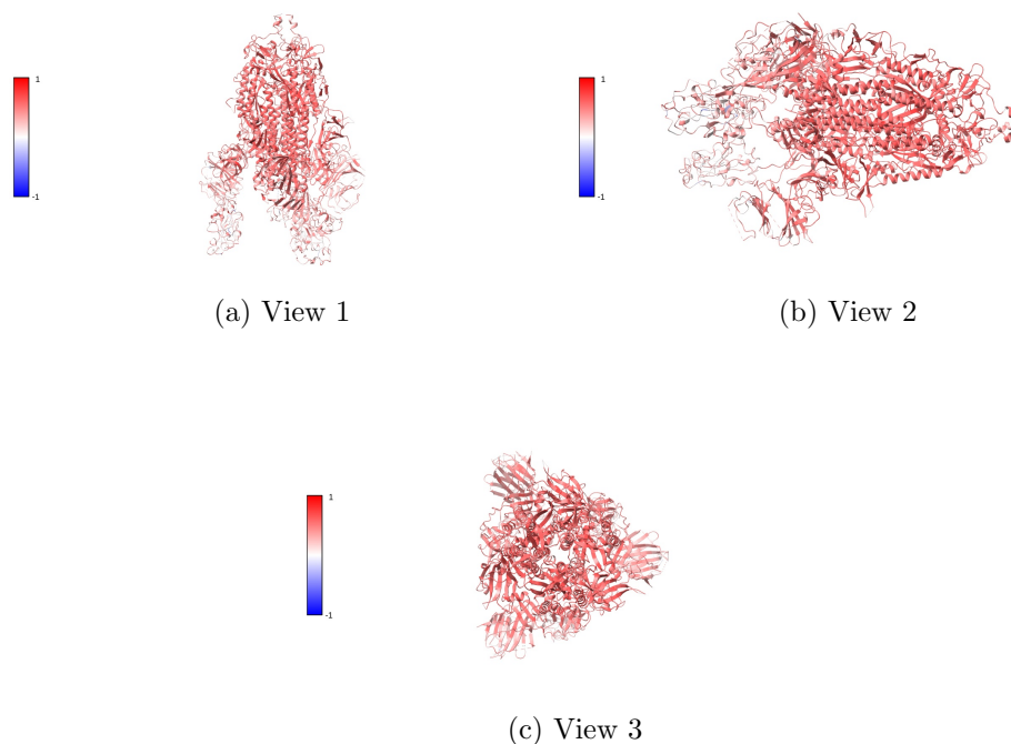
Figure 17: Atomic model colored by MapQ Views generated by ChimeraX at a the following X, Y, Z angles: View 1 (0, -90, -90), View 2 (-90, 0, -90), View 3 (0, 0, 0).
