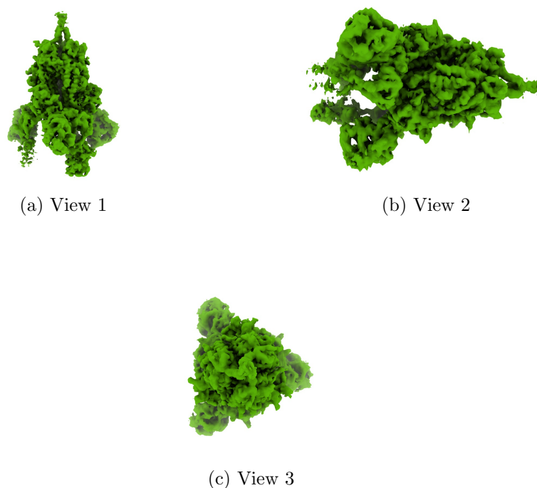
Figure 4: Isosurface at threshold=0.800000. Views generated by ChimeraX at a the following X, Y, Z angles: View 1 (0, -90, -90), View 2 (-90, 0, -90), View 3 (0, 0, 0).
