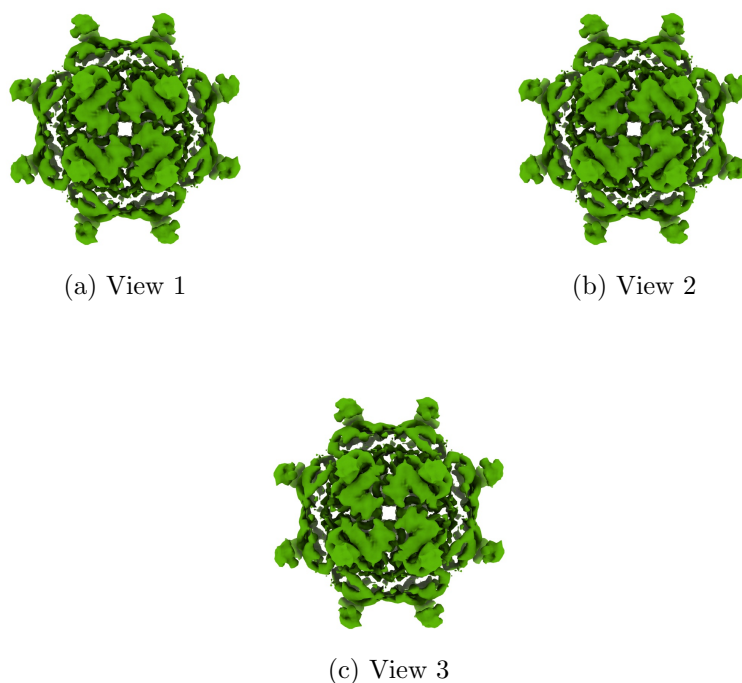
Figure 4: Isosurface at threshold=0.007130. Views generated by ChimeraX at a the following X, Y, Z angles: View 1 (0, -90, -90), View 2 (-90, 0, -90), View 3 (0, 0, 0).
