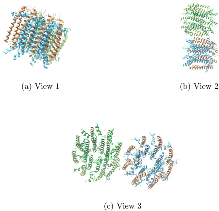
Figure 10: Input atomic model Views generated by ChimeraX at the following X, Y, Z angles: View 1 (0, -90, -90), View 2 (-90, 0, -90), View 3 (0, 0, 0).
