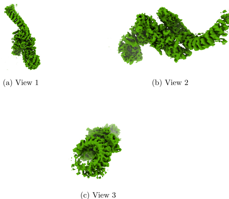
Figure 4: Isosurface at threshold=0.580000. Views generated by ChimeraX at a the following X, Y, Z angles: View 1 (0, -90, -90), View 2 (-90, 0, -90), View 3 (0, 0, 0).
