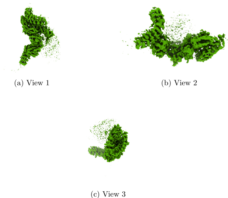
Figure 4: Isosurface at threshold=0.670000. Views generated by ChimeraX at a the following X, Y, Z angles: View 1 (0, -90, -90), View 2 (-90, 0, -90), View 3 (0, 0, 0).
