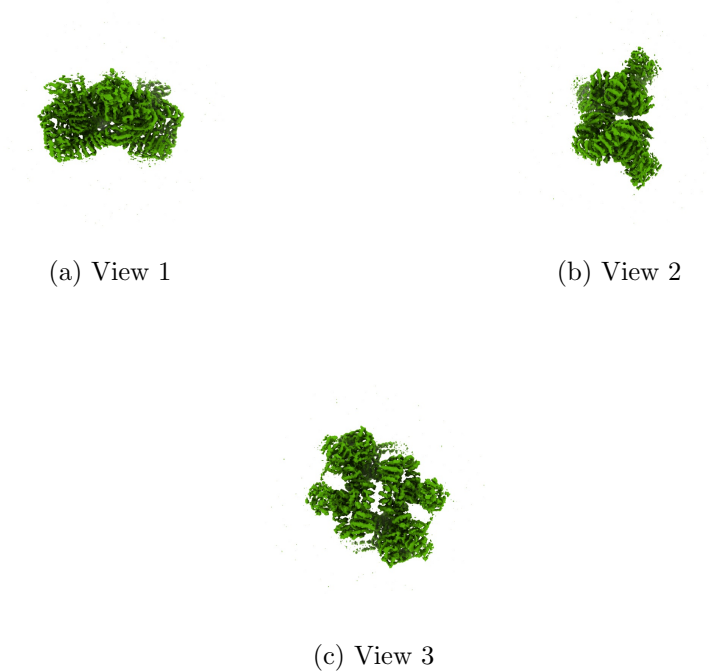
Figure 4: Isosurface at threshold=4.180000. Views generated by ChimeraX at a the following X, Y, Z angles: View 1 (0, -90, -90), View 2 (-90, 0, -90), View 3 (0, 0, 0).
