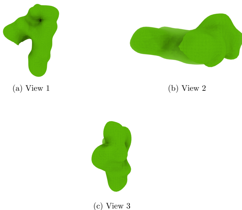
Figure 4: Isosurface at threshold=2.170000. Views generated by ChimeraX at a the following X, Y, Z angles: View 1 (0, -90, -90), View 2 (-90, 0, -90), View 3 (0, 0, 0).
