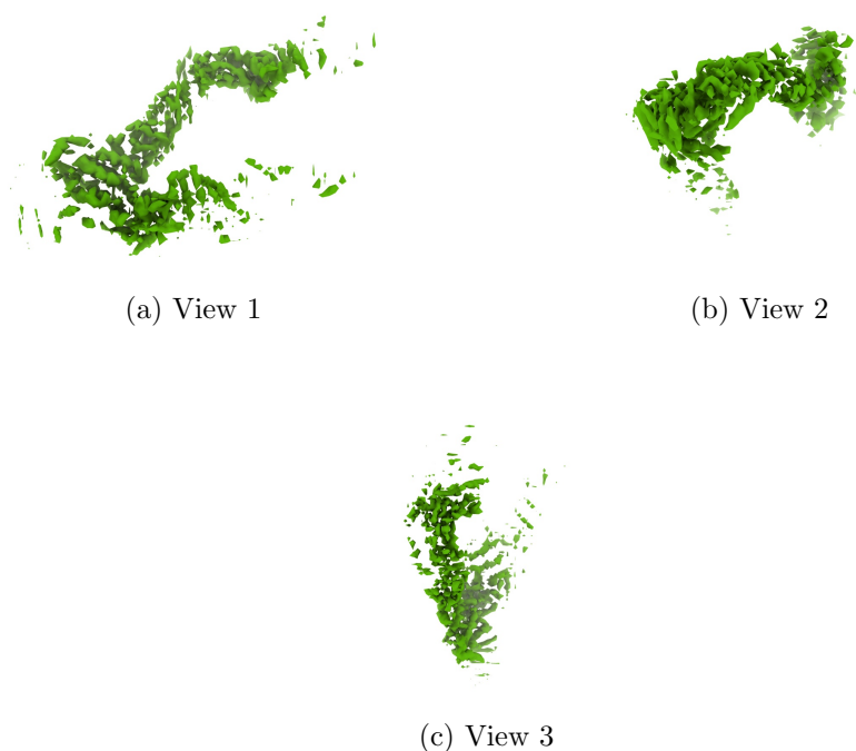
Figure 4: Isosurface at threshold=0.040000. Views generated by ChimeraX at a the following X, Y, Z angles: View 1 (0, -90, -90), View 2 (-90, 0, -90), View 3 (0, 0, 0).
