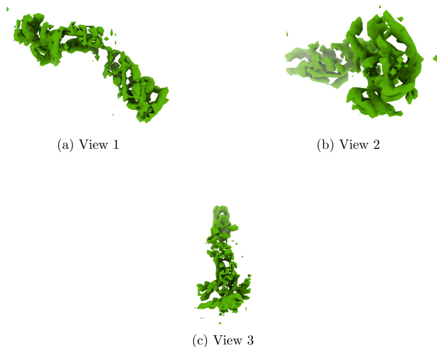
Figure 4: Isosurface at threshold=0.040000. Views generated by ChimeraX at a the following X, Y, Z angles: View 1 (0, -90, -90), View 2 (-90, 0, -90), View 3 (0, 0, 0).
