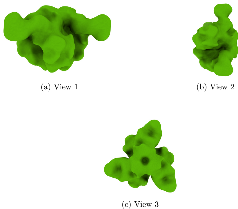
Figure 4: Isosurface at threshold=0.012300. Views generated by ChimeraX at a the following X, Y, Z angles: View 1 (0, -90, -90), View 2 (-90, 0, -90), View 3 (0, 0, 0).
