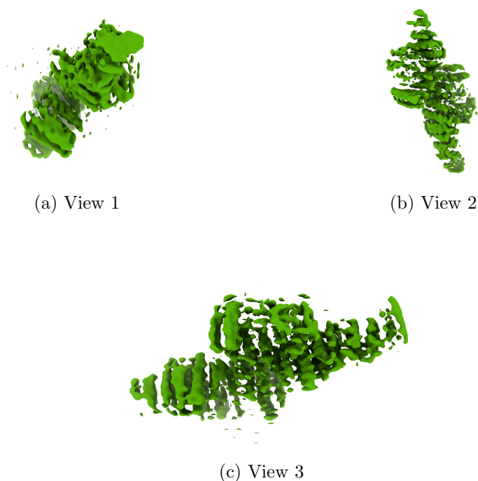
Figure 4: Isosurface at threshold=0.024400. Views generated by ChimeraX at a the following X, Y, Z angles: View 1 (0, -90, -90), View 2 (-90, 0, -90), View 3 (0, 0, 0).
