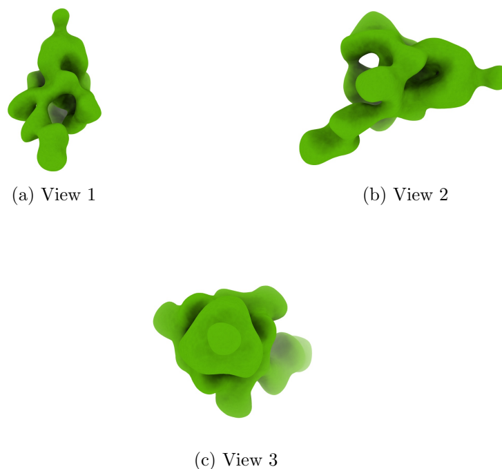
Figure 4: Isosurface at threshold=0.027400. Views generated by ChimeraX at a the following X, Y, Z angles: View 1 (0, -90, -90), View 2 (-90, 0, -90), View 3 (0, 0, 0).
