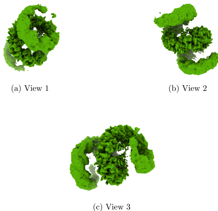
Figure 4: Isosurface at threshold=0.082700. Views generated by ChimeraX at a the following X, Y, Z angles: View 1 (0, -90, -90), View 2 (-90, 0, -90), View 3 (0, 0, 0).
