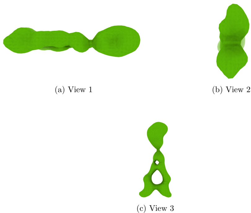
Figure 4: Isosurface at threshold=2.400000. Views generated by ChimeraX at a the following X, Y, Z angles: View 1 (0, -90, -90), View 2 (-90, 0, -90), View 3 (0, 0, 0).
