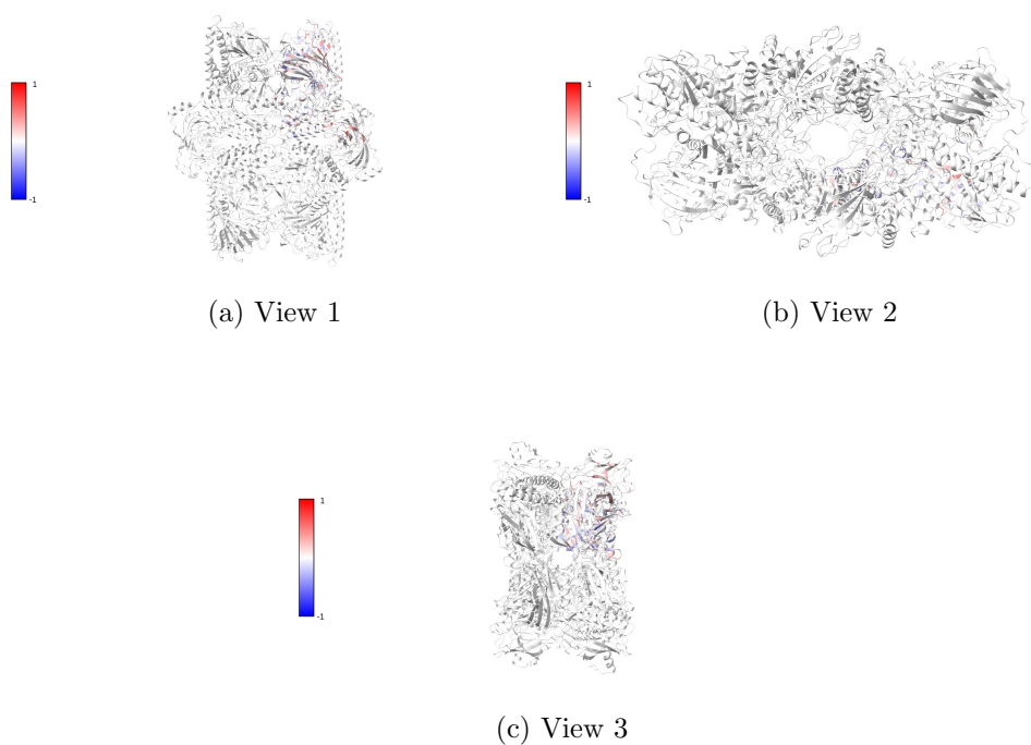
Figure 23: Atomic model colored by MapQ Views generated by ChimeraX at a the following X, Y, Z angles: View 1 (0, -90, -90), View 2 (-90, 0, -90), View 3 (0, 0, 0).
