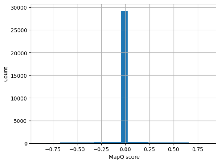
Figure 22: Histogram of the per-atom Q-score.
