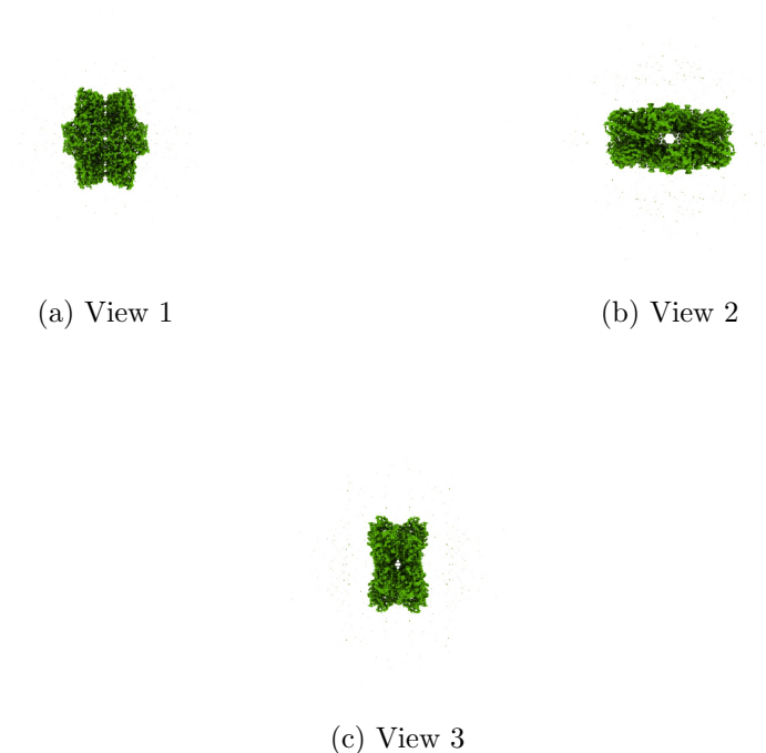
Figure 4: Isosurface at threshold=4.500000. Views generated by ChimeraX at a the following X, Y, Z angles: View 1 (0, -90, -90), View 2 (-90, 0, -90), View 3 (0, 0, 0).
