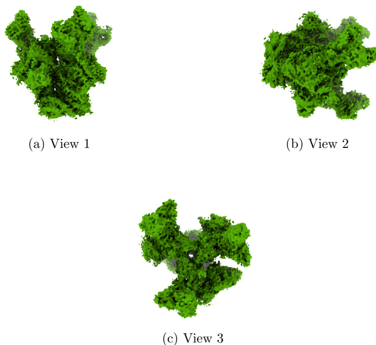
Figure 4: Isosurface at threshold=0.007310. Views generated by ChimeraX at a the following X, Y, Z angles: View 1 (0, -90, -90), View 2 (-90, 0, -90), View 3 (0, 0, 0).
