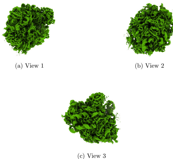
Figure 4: Isosurface at threshold=0.019200. Views generated by ChimeraX at a the following X, Y, Z angles: View 1 (0, -90, -90), View 2 (-90, 0, -90), View 3 (0, 0, 0).
