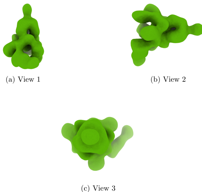
Figure 4: Isosurface at threshold=0.010100. Views generated by ChimeraX at a the following X, Y, Z angles: View 1 (0, -90, -90), View 2 (-90, 0, -90), View 3 (0, 0, 0).
