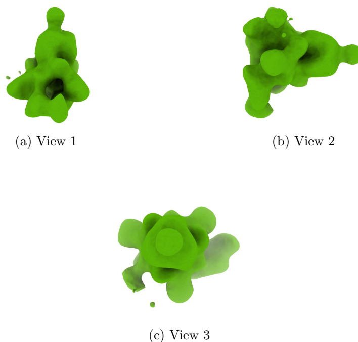
Figure 4: Isosurface at threshold=0.007870. Views generated by ChimeraX at a the following X, Y, Z angles: View 1 (0, -90, -90), View 2 (-90, 0, -90), View 3 (0, 0, 0).
