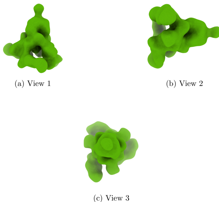
Figure 4: Isosurface at threshold=0.009100. Views generated by ChimeraX at a the following X, Y, Z angles: View 1 (0, -90, -90), View 2 (-90, 0, -90), View 3 (0, 0, 0).
