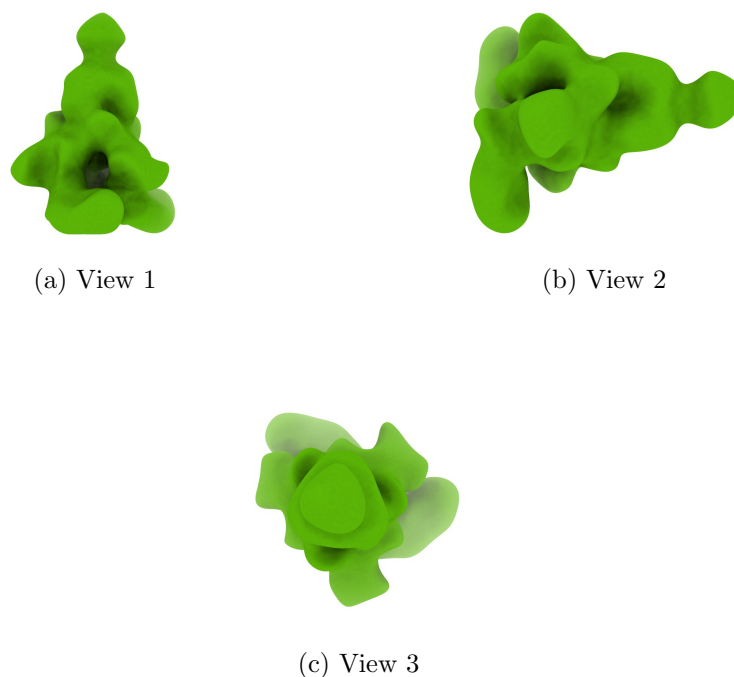
Figure 4: Isosurface at threshold=0.005700. Views generated by ChimeraX at a the following X, Y, Z angles: View 1 (0, -90, -90), View 2 (-90, 0, -90), View 3 (0, 0, 0).
