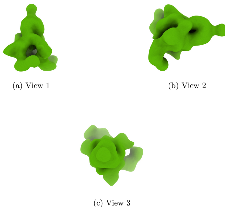
Figure 4: Isosurface at threshold=0.010400. Views generated by ChimeraX at a the following X, Y, Z angles: View 1 (0, -90, -90), View 2 (-90, 0, -90), View 3 (0, 0, 0).
