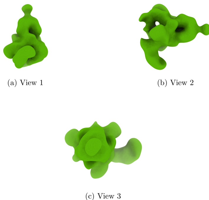
Figure 4: Isosurface at threshold=0.017200. Views generated by ChimeraX at the following X, Y, Z angles: View 1 (0, -90, -90), View 2 (-90, 0, -90), View 3 (0, 0, 0).
