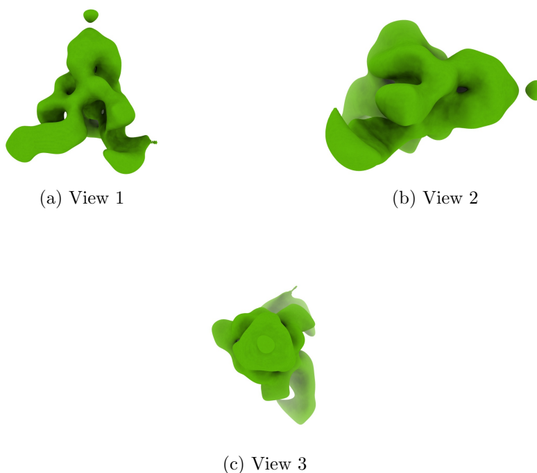
Figure 4: Isosurface at threshold=0.028900. Views generated by ChimeraX at a the following X, Y, Z angles: View 1 (0, -90, -90), View 2 (-90, 0, -90), View 3 (0, 0, 0).
