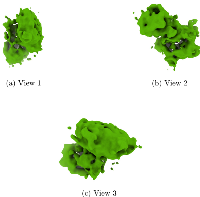
Figure 4: Isosurface at threshold=0.900000. Views generated by ChimeraX at a the following X, Y, Z angles: View 1 (0, -90, -90), View 2 (-90, 0, -90), View 3 (0, 0, 0).
