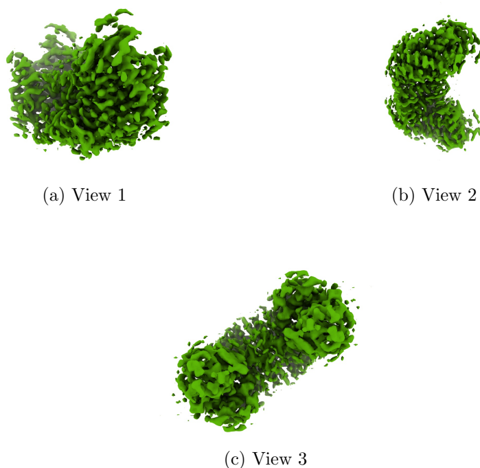
Figure 4: Isosurface at threshold=0.365000. Views generated by ChimeraX at a the following X, Y, Z angles: View 1 (0, -90, -90), View 2 (-90, 0, -90), View 3 (0, 0, 0).
