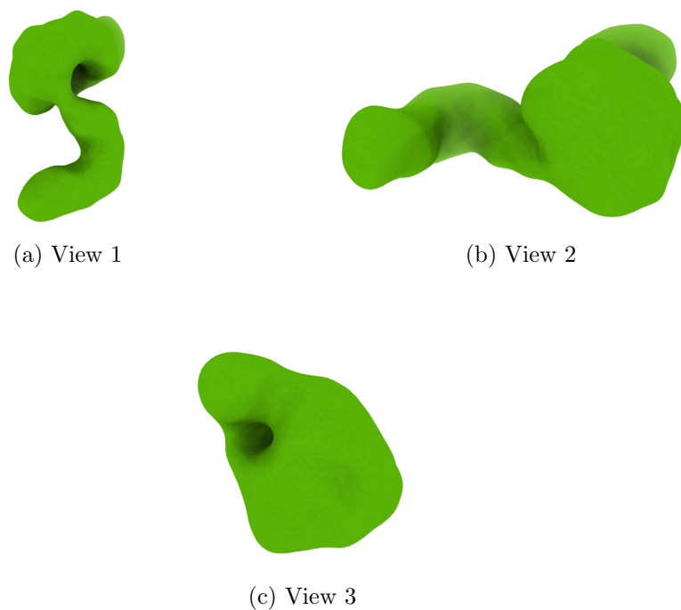
Figure 4: Isosurface at threshold=3.520000. Views generated by ChimeraX at a the following X, Y, Z angles: View 1 (0, -90, -90), View 2 (-90, 0, -90), View 3 (0, 0, 0).
